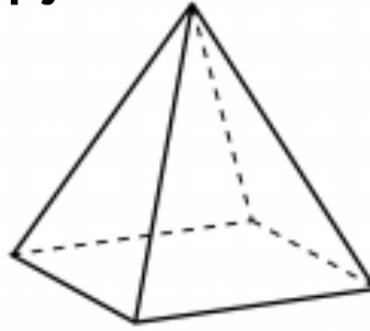
square-based pyramid
