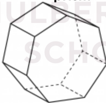
heptagonal prism
