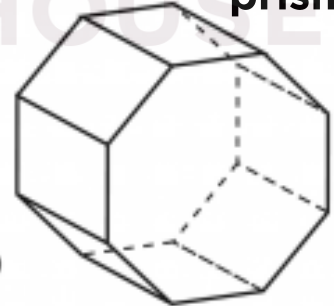
octagonal prism
