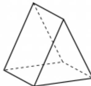
triangular prism
