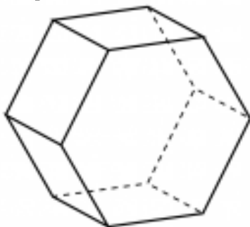
hexagonal prism
