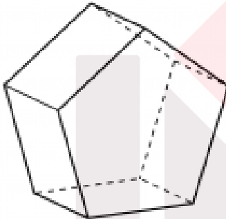
pentagonal prism
