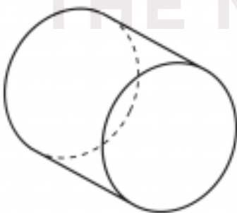
cylinder
